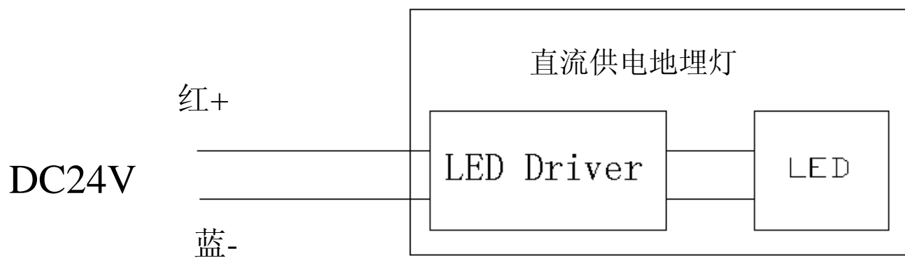
Wiring circuit
